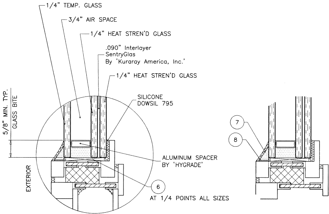
GLAZING DETAIL 1-1/2" OVERALL INSUL. LAM. GLASS
